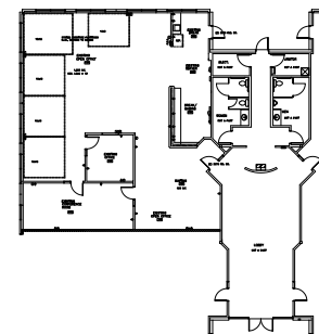
FLOOR PLAN
