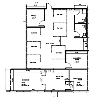
FLOOR PLAN
